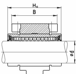
PTO Housing Unit
